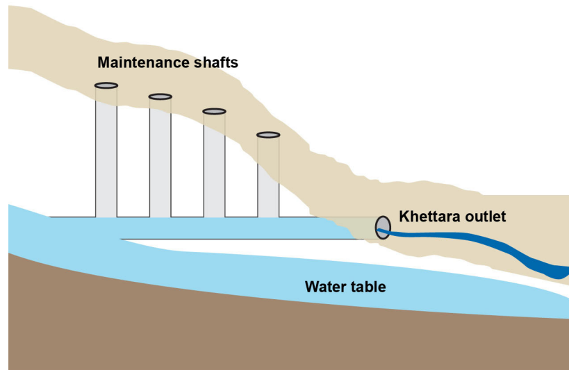
Figure V.2. Khattara structure
